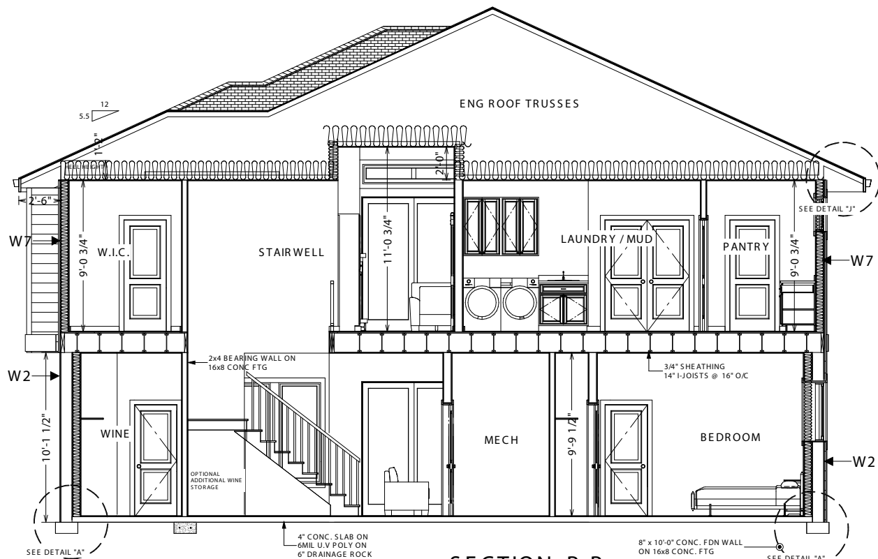
SECTION B-B
